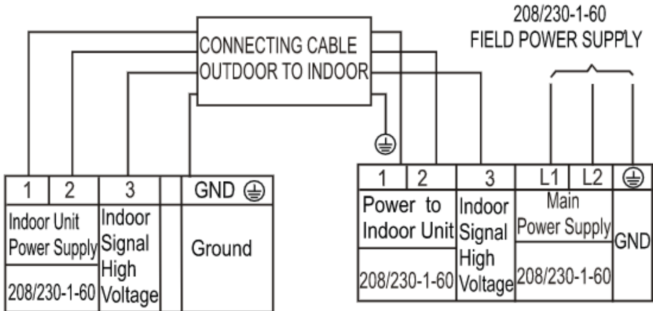
Fig. 7 — Wiring Diagram (All Sizes)
