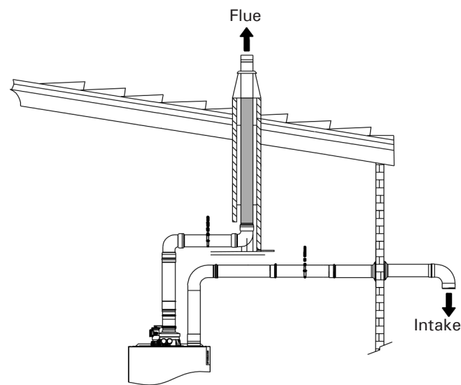
Flexible two pipe system (room air independent)
