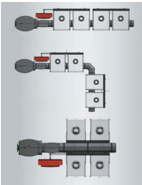
The prefabricated distribution manifold is available in a variety of configurations: single-line, corner or back-to-back.
