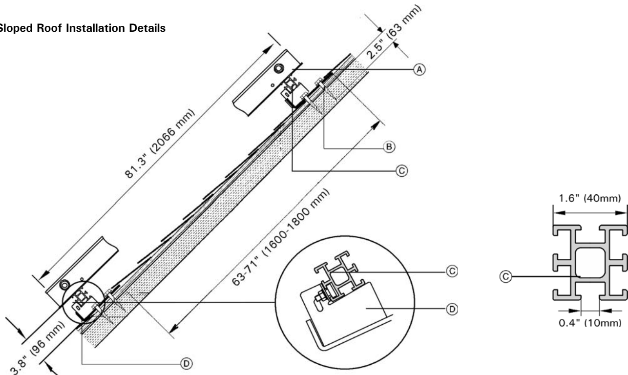
Roof bracket for shingled roofs
