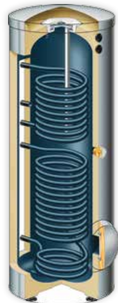
Vitocell 100-B dual-coil storage tank
