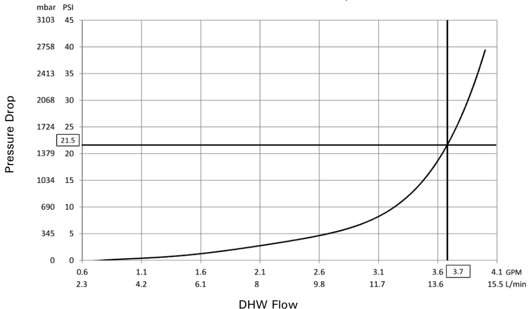
BiKA - 35 DHW Pressure Drop
